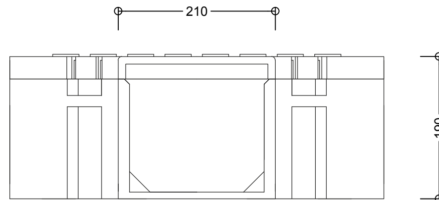
Elevation View
