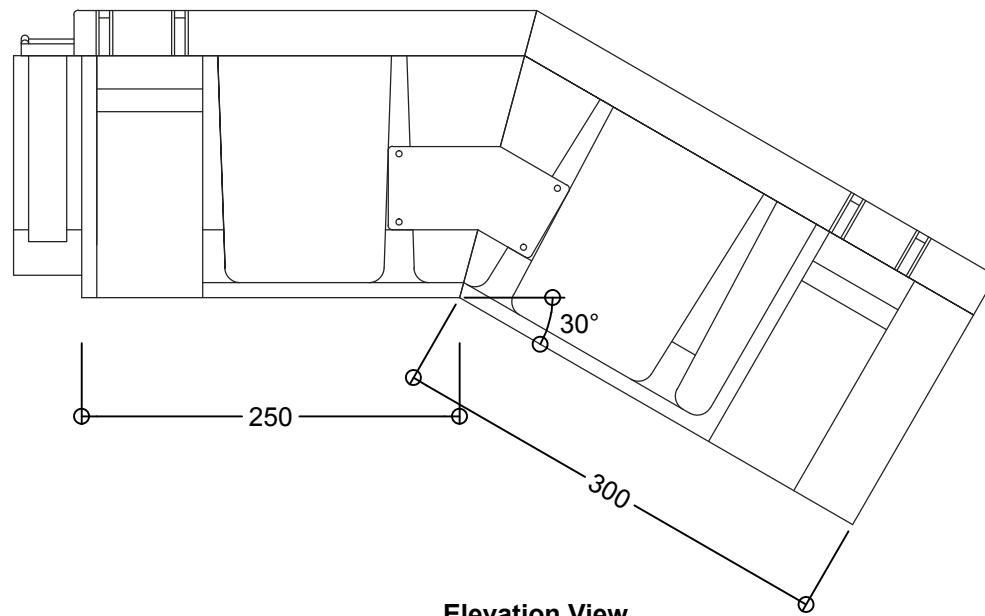
Elevation View
