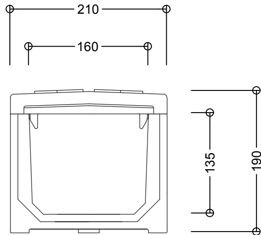
Section View
